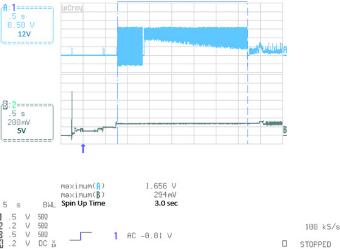
Figure 2 Typical 12V startup and operation current profile (1 and 2-disk models)
