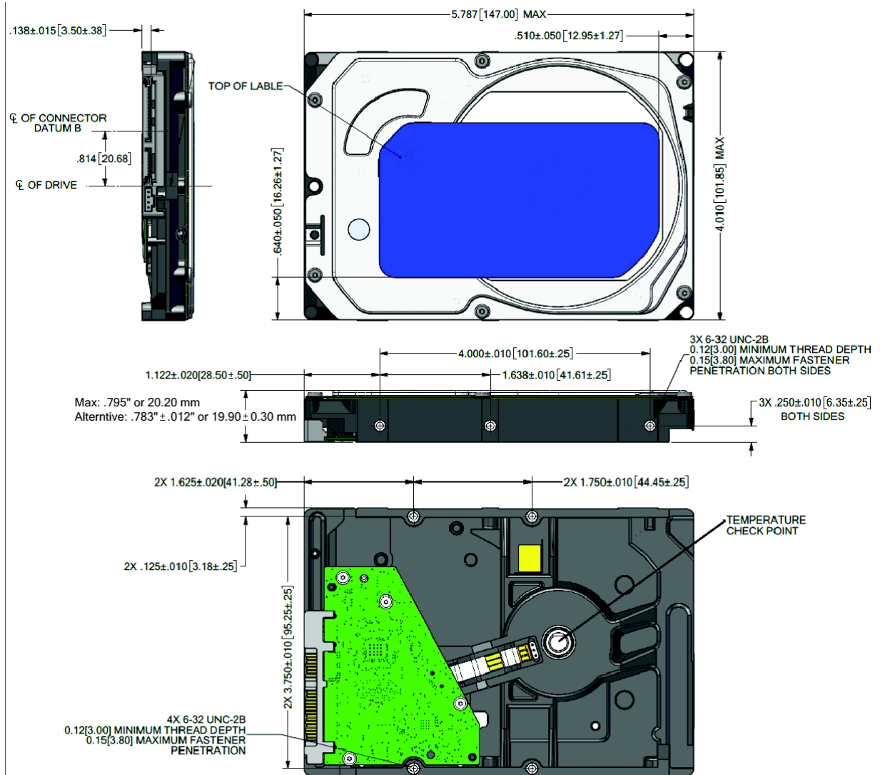
Figure 4 Mounting dimensions (4TB, 3TB, 2TB & 1TB models)
