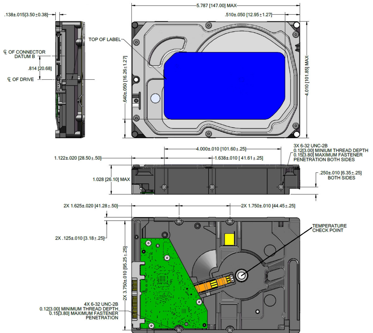
Figure 5 Mounting dimensions (8TB & 6TB models)
