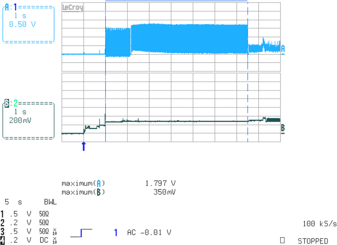
Figure 1 Typical 12V startup and operation current profile (4-disk models)
