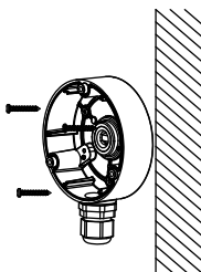
Figure 2-6 Secure Junction Box on Wall
