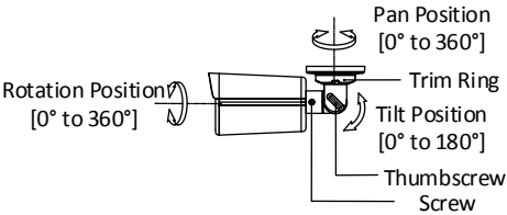
Figure 2-3 3-Axis Adjustment
