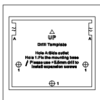
Figure 2-9 Drill Template for Wall Mount
