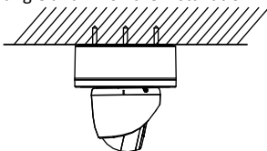
Figure 2-25 Finish Installation
