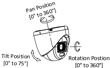
Figure 2-21 3-Axis Adjustment
