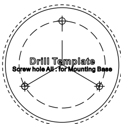
Figure 2-17 Drill Template
