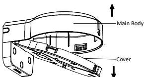
Figure 2-8 Take Apart Wall Mount
