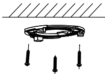
Figure 2-18 Attach Gang Box to Ceiling
