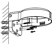
Figure 2-66 Secure Main Body to Wall
