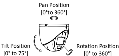
Figure 2-39 3-Axis Adjustment
