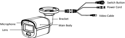
Figure 1-1 Overview of Type I Camera
