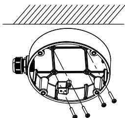
Figure 2-59 Secure Junction Box Body
