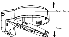
Figure 2-64 Take Apart Wall Mount
