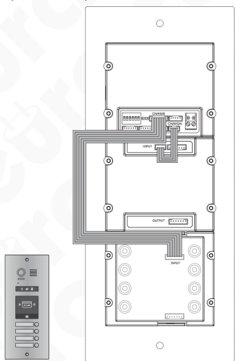
Fig. 45. Connection diagram of the main module, proximity card reader and call buttons
