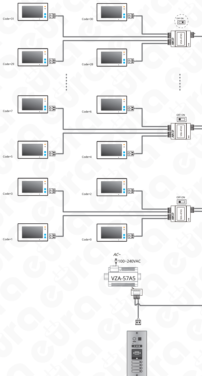
Fig. 7. Connection diagram of a modular cassette with monitors using the VXA-47A5 signal distributor
