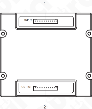
Fig. 21. VXA-64A5 Encryptor Keyboard Module Terminals
