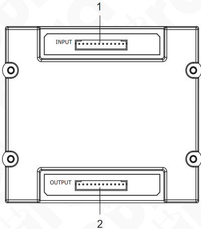
Fig. 21. VXA-64A5 Encryptor Keyboard Module Terminals
