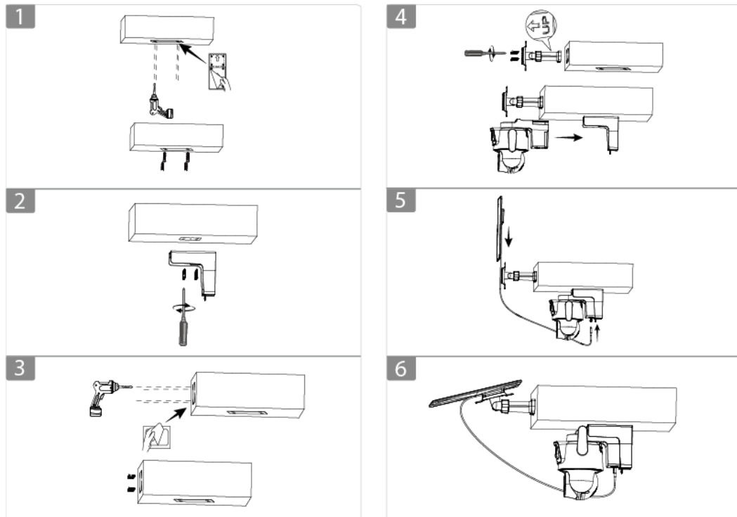
Figure 4-6 Pole mount installation
