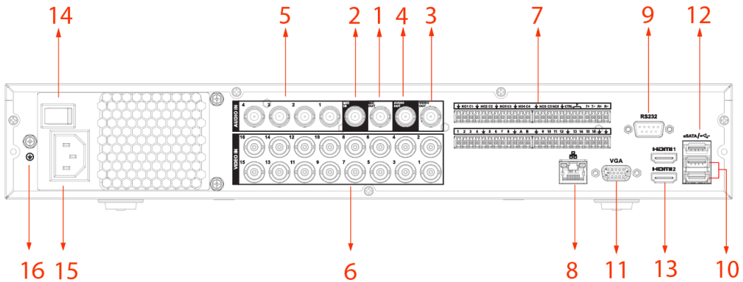
Figure 3-21 Rear panel (3)
