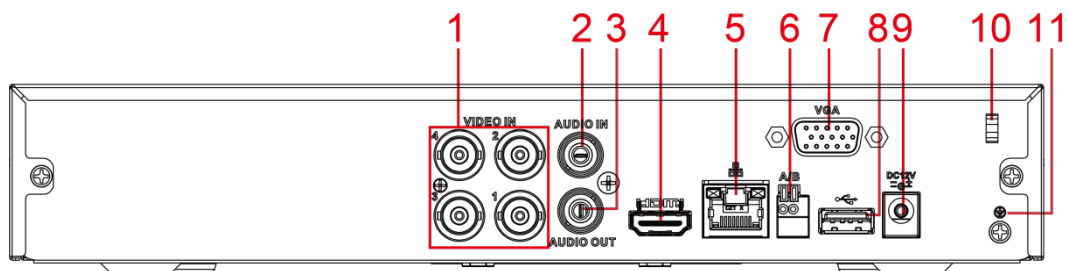
Figure 3-14 Rear panel
